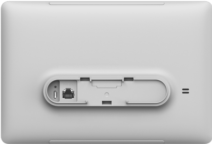
Above: The I/O section of Cisco Room Navigator for Table with the foot stand deattached from the touch panel.
